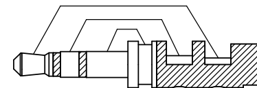
CONTACT DIAGRAM
