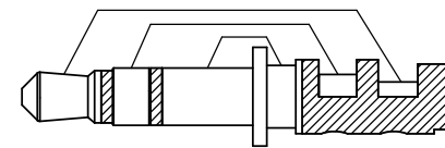
CONTACT DIAGRAM
